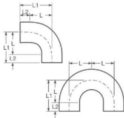
DIMENSIONS OF 90° AND 180° TUBE BENDS millimetres
