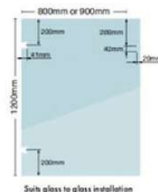
Suits glass to glass installation
