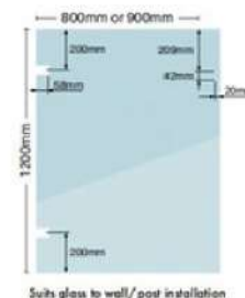
Suits glass to wall/post installation
